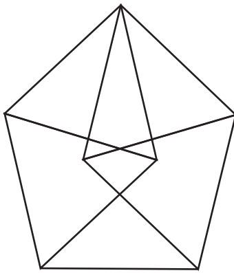
Figure 2: Proof that 4 \leq \chi(\mathbb{E}^2) .
