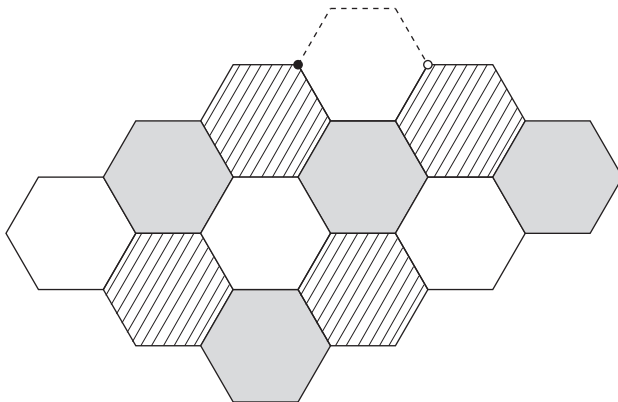
Figure 1: A sketch of the 3-coloring avoiding the (a, a, 2a) triangle.
